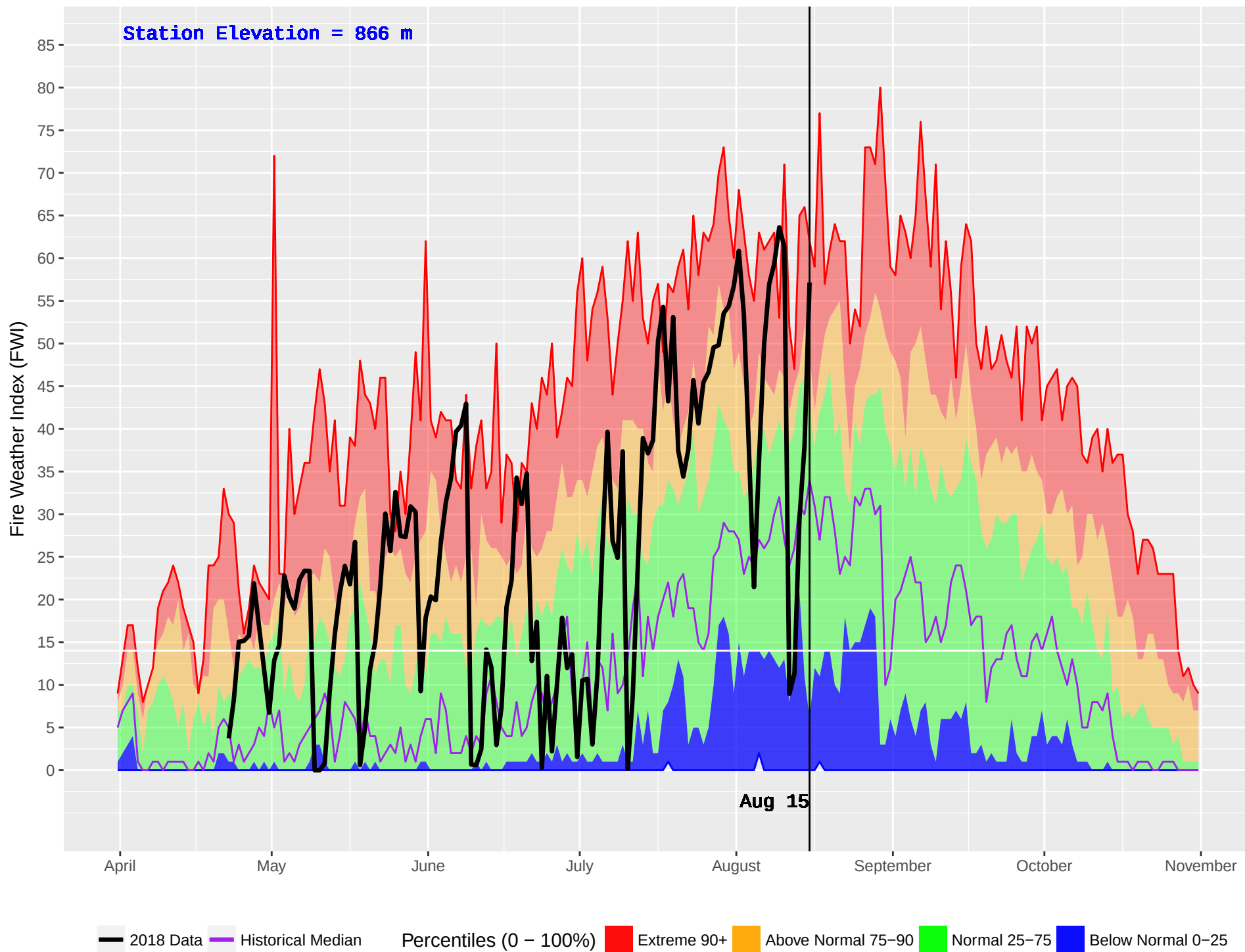
NICOLL (393) : Historical (1981–2016) and Current (2018) Daily Fire Weather Index (FWI)
