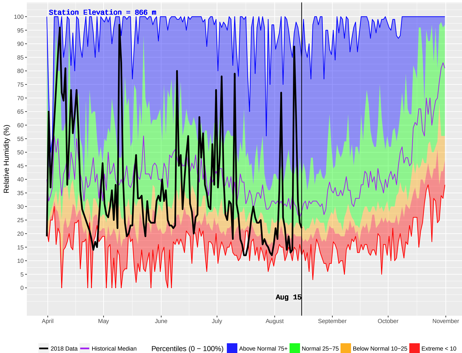
NICOLL (393) : Historical (1981–2016) and Current (2018) Daily Relative Humidity
