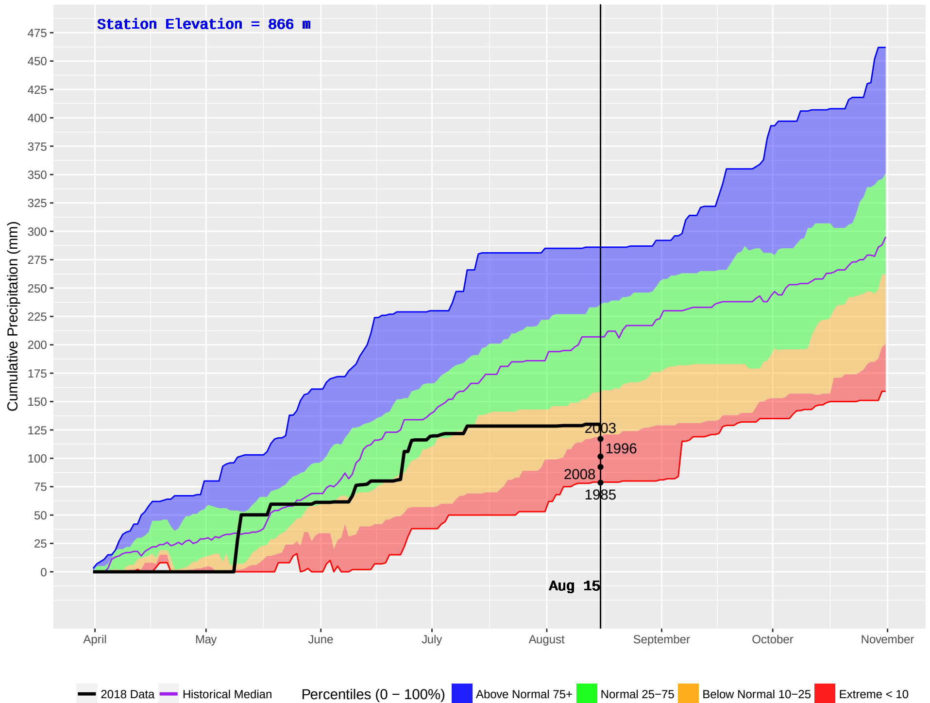
NICOLL (393) : Historical (1981–2016) and Current (2018) Daily Cumulative Precipitation
